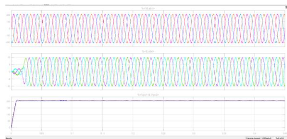
Fig.8 a) Simulation results for load and weather variation when the SOC is superior to 50%, and b) zoomed responses of (a) between t = 0.35s and t=0.6s
