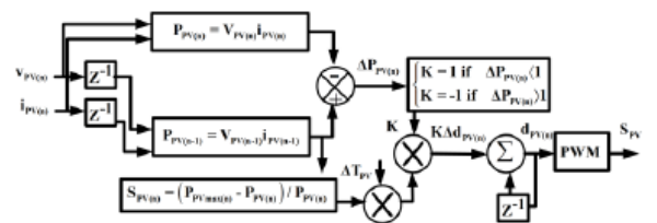
Fig. 3. Control scheme for MPPT from PV
