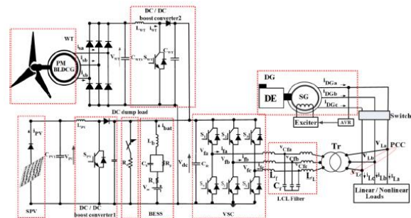
Fig.1 SMG configuration under study
